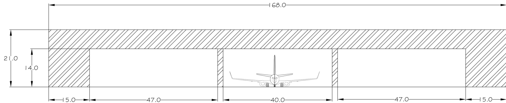
PROFILE VIEW
